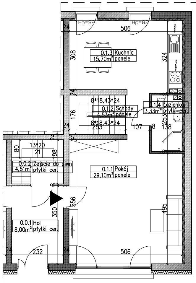
PARTER - 52,66m 2
